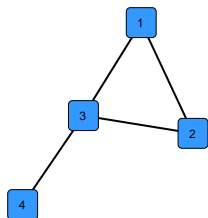
(a) G_{t=1}
