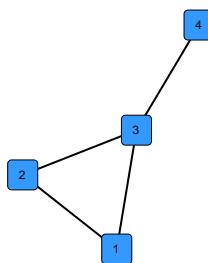
(a) G_{t=1}
