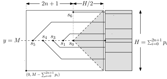
Fig. 5: For each job J_j , i = 0, 1, \dots, 2n we introduce a site s_i placed at (2n + 1 - i, M) .
