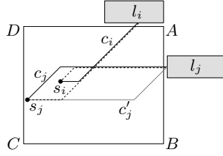
Fig. 12: An instance that does not have a valid labeling with do - and pd -leaders.
