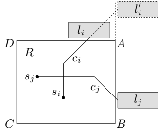
Fig. 13: An od -leader to the top side of R is extended into a pd -leader to the right side of R .
