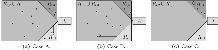
Fig. 19: Illustration of the different cases of Algorithm 2.
