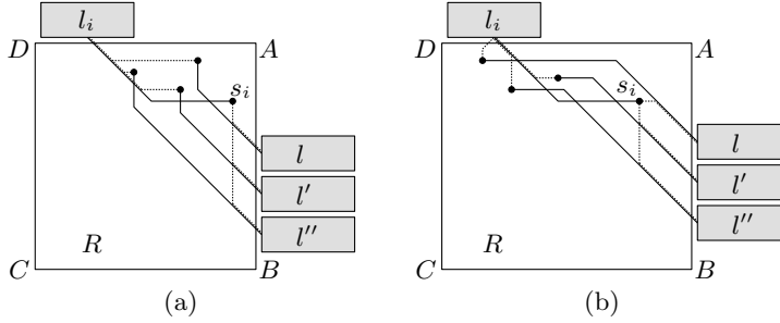
Fig. 14: Two intersecting pd -leaders (a) and a pair of intersecting pd - and od -leaders (b) directed towards D and B can be shortened by swapping the label assignment.
