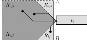
Fig. 4: Connecting site s_i to label l_i .
