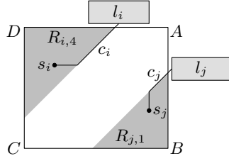
Fig. 15: Two pd -leaders towards corner A cannot intersect.
