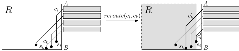
Fig. 9: Rerouting the crossing pd -leaders c_i and c_k .
