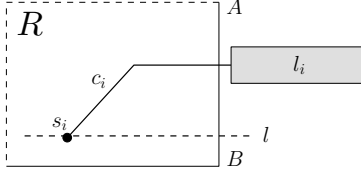
Fig. 3: c_i is oriented towards corner A .
