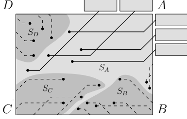
Fig. 16: Sets S_A , S_B , S_C and S_D .
