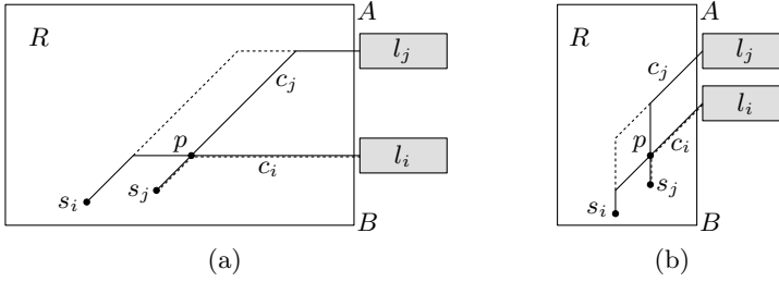
Fig. 8: Swapping two crossing leaders removes the crossing and keeps the total length.
