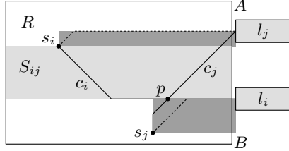
Fig. 6: The total length of two oppositely directed leaders can be decreased. The bounding boxes of the new (dotted) leaders are shaded in dark gray.
