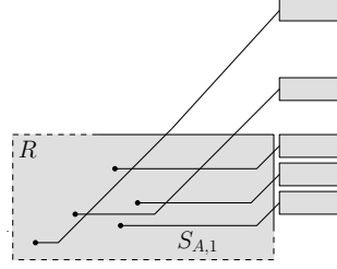
Fig. 17: Extending a pd -leader
